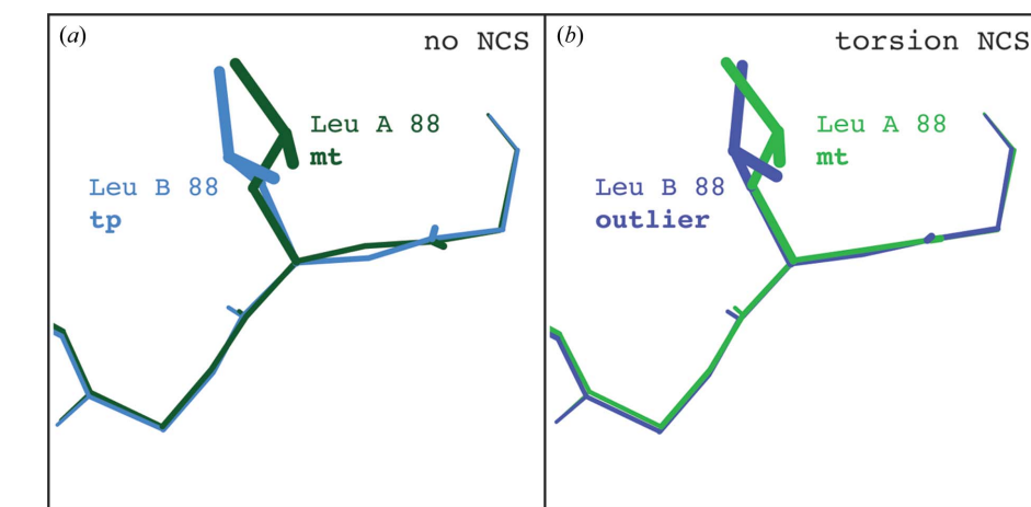
Figure 7 Comparison of NCS-related LeuA88 and LeuB88 of PDB entry 1jbb refined with and without torsion NCS restraints. (a) Refinement without NCS restraints allows the incorrectly built LeuB88 side chain to remain a tp rotamer while distorting the surrounding backbone geometry. (b) Refinement using torsion NCS restraints preserves similar backbone geometry, which causes the incorrectly built LeuB88 side chain to present as an outlier. Images were generated using KiNG (Chen et al. , 2009).
